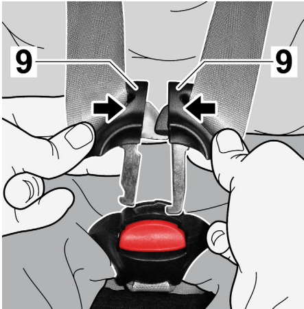
5. Bring the belt tongues (9) together
